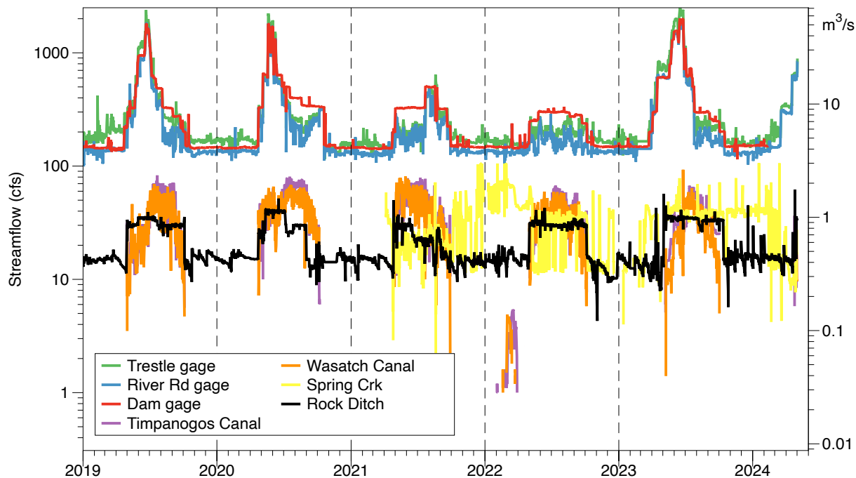
Figure 2217. 2019-2024 discharge measurements at the three streamflow gauges on the Middle Provo River (Dam, River Road and Trestle), the Spring Creek tributary, and the three (Timpanogos canal, Wasatch canal and Rock Creek ditch) irrigation diversions. Data from CUWCD and USGS.
