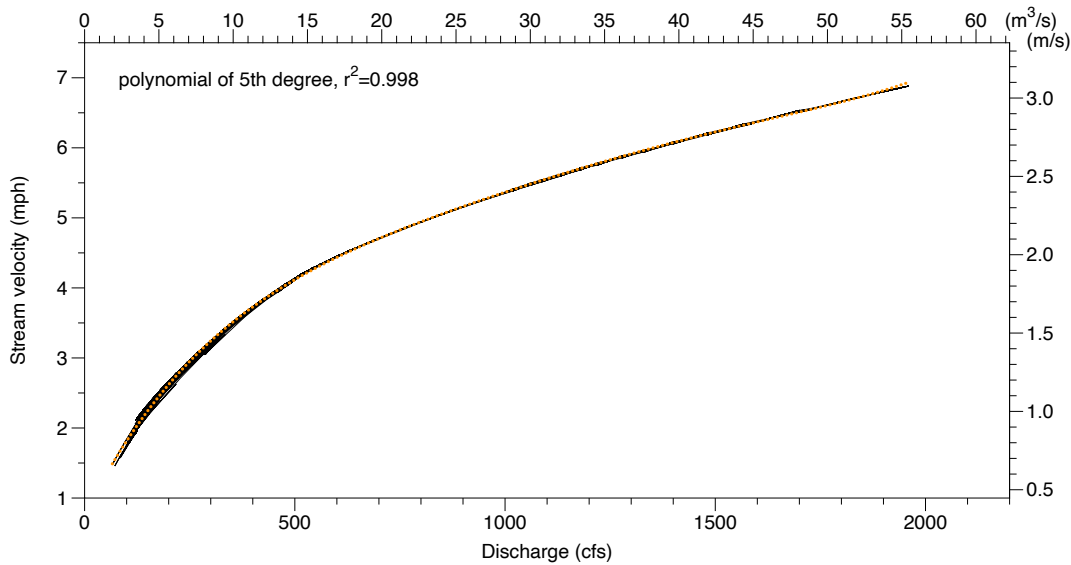
Figure 16. Stream velocity as a function of discharge at the River Road Bridge. Data from USGS.
