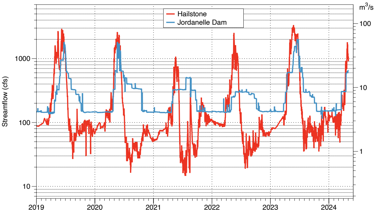
Figure 6. Upper Provo River streamflow entering the Jordanelle Reservoir at the USGS Hailstone gauge (red) compared to water releases from the Jordanelle Reservoir (blue) during the period 2019-2024. Note the logarithmic scale. Data from USGS and CUWCD.
