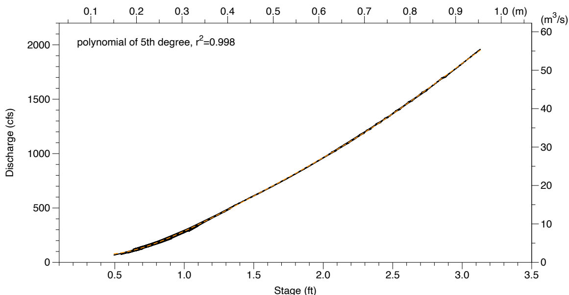
Figure 15. Discharge as a function of stage at the River Road Bridge gage. Data from USGS
